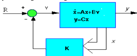
Fig. 3. State variable feedback with K.
