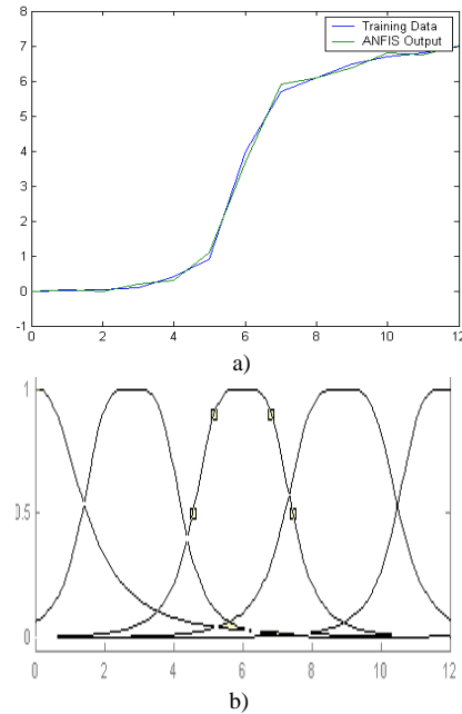
a) Five Bell shaped member functions. b) The nonlinear function is modeled.
