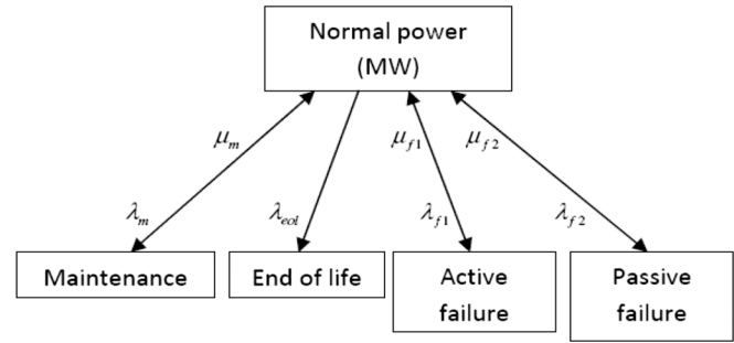
Fig. 1. Reliability model for the generator, transformer, and circuit breaker.
