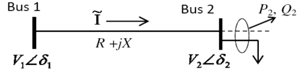
Fig. 7. Simple two-bus distribution system [24].
