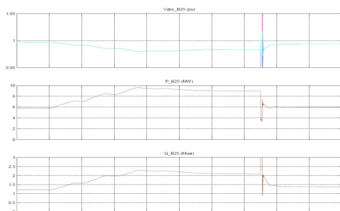
Fig. 8. Voltages, Active and Reactive Power at B25 Bus
