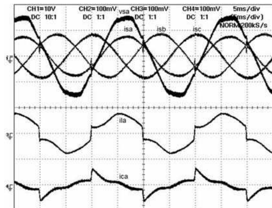
Fig. 20. Load unbalance compensation. Traces from top to bottom: source voltage (phase a), v_{sar} (100 V/div); source currents, i_{sar} , i_{sb} , i_{sc} (10 A/div); load current, i_{lar} (10 A/div); filter current, i_{car} (10 A/div).
