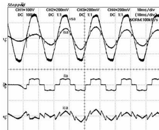
Fig. 19. Transient compensation of a three-phase diode rectifier. Traces from top to bottom (phase a): source voltage, v_{sar} (100 V/div); source current, i_{sar} (20 A/div); load current, i_{lar} (20 A/div); filter current, i_{car} (20 A/div).
