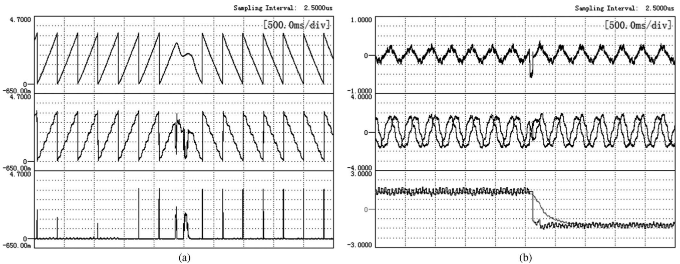
Fig. 15. Operating waveforms when the reference speed is changed from +15 to -15\text{ r/min} . (a) From top to bottom are the actual rotor position, estimated rotor position, and estimated error ( 67.8^\circ/\text{div} ), respectively. (b) From top to bottom are the A-phase stator current ( 3.8\text{ A/div} ), the estimated back EMF ( 13\text{ V/div} ), and the actual and the estimated speed ( 8.5\text{ r/min/div} ), respectively.
