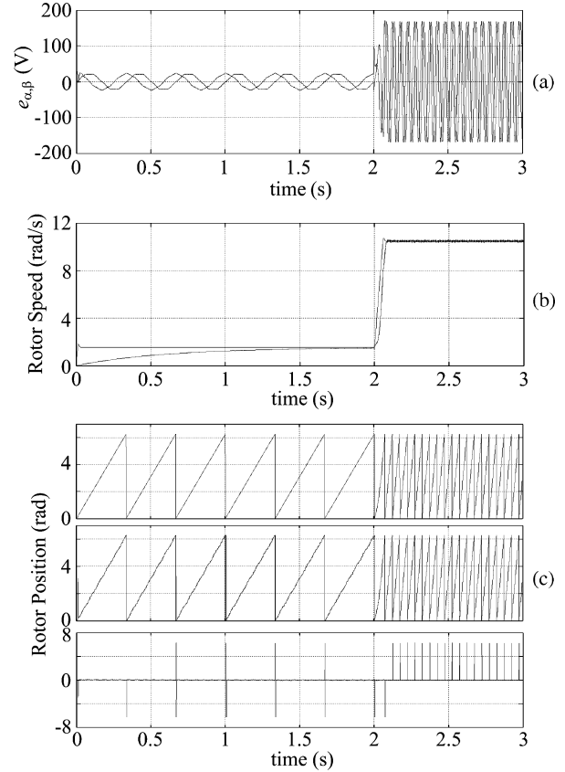
Fig. 7. Simulation waveforms when l = 300 . (a) Estimated back EMF. (b) Actual and estimated speeds. (c) Actual rotor position, estimated rotor position, and estimated error.
