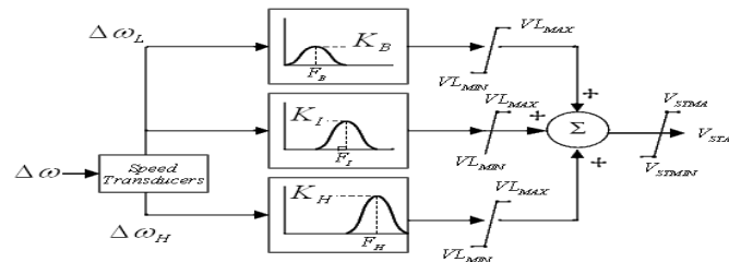
Figure 2. The Block Diagram of the Multi-band Power System Stabilizer (MB-PSS)
