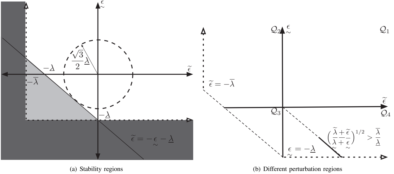
Fig. 1. Perturbations in the white and gray area correspond to the stable and unstable regions of multi-step algorithm respectively. (b) Multi-step algorithm outperforms gradient iterations in (\varepsilon, \tilde{\varepsilon}) \in \mathcal{C} \setminus \mathcal{Q}_4 . For symmetric errors in \mathcal{Q}_4 (along the line \tilde{\varepsilon} = -\varepsilon ) gradient might outperform multi-step algorithm.
