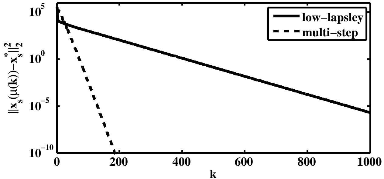
Fig. 5. Convergence of Low-Lapsley and multi-step. Plot shows log scale of the Euclidian distance from optimal source rates \|x_s(\mu(k)) - x_s^*\|_2^2 vs. the iteration number k .
