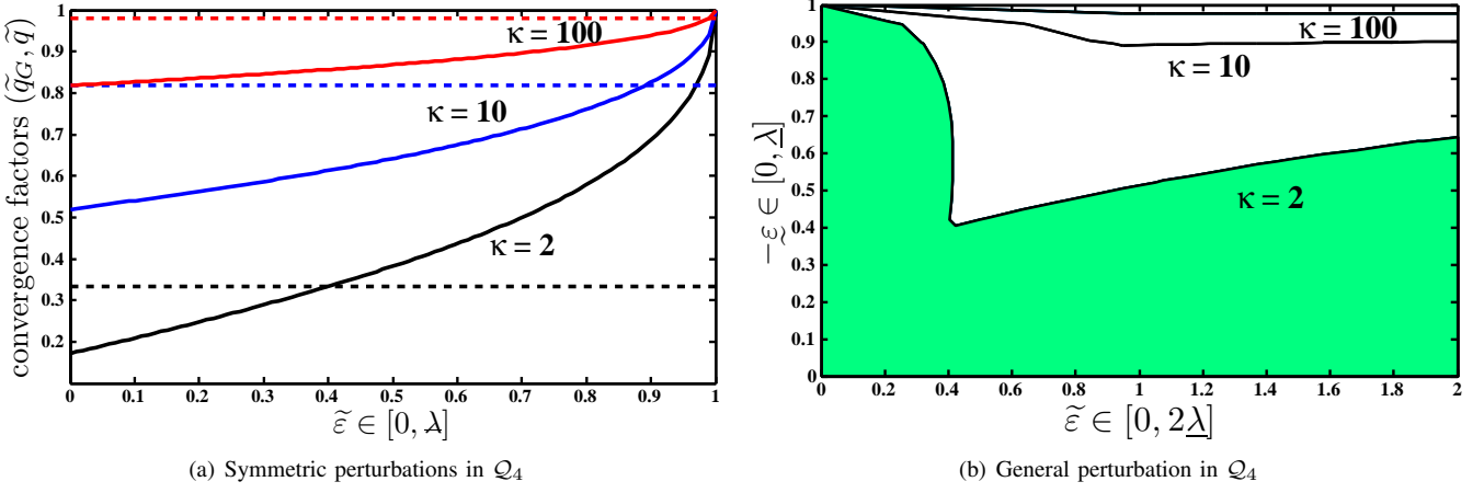
Fig. 2. (a) Convergence factor of multi-step and gradient algorithms under the condition described by (19). Solid lines belong to \tilde{q} while the dashed lines depict \tilde{q}_G . (b) Level curves of \tilde{q} - \tilde{q}_G around the origin for (\varepsilon, \tilde{\varepsilon}) \in \mathcal{Q}_4 .
