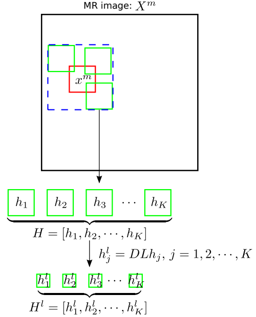
Fig. 1. Hypothesis generation within a search window.
