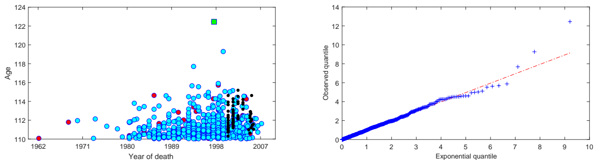
Figure 4: IDL data with validation level A, from “World”. Left : Life lengths against year of death: blue women, red men, black persons who died after December 31, 1999 in USA or after August 31, 2003 in Japan and which are not included in analyses. Green square is Jeanne Calment. Right : Empirical quantiles plotted against quantiles of exponential distribution with the estimated mean. For an impression of the statistical variation of such plots, see Fig. 5.
