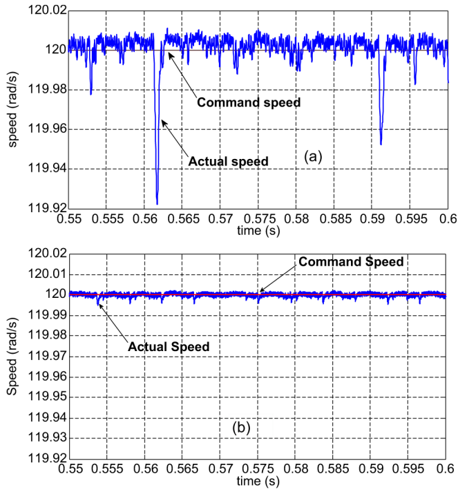
Fig. 8. Steady-state speed responses of the IM drive for a step change in load from 0.3 to 0.8 N · m at 120 rad/s. (a) Conventional DTC. (b) FLC-based DTC.
