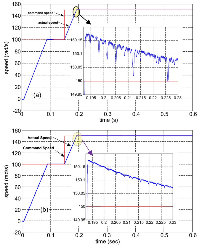
Fig. 10. Speed responses of the IM drive with zoom-in view of the encircled portion of the response, for a step change in command speed from 100 to 150 rad/s at a 0.5-N · m load. (a) Conventional DTC. (b) FLC-based DTC scheme.
