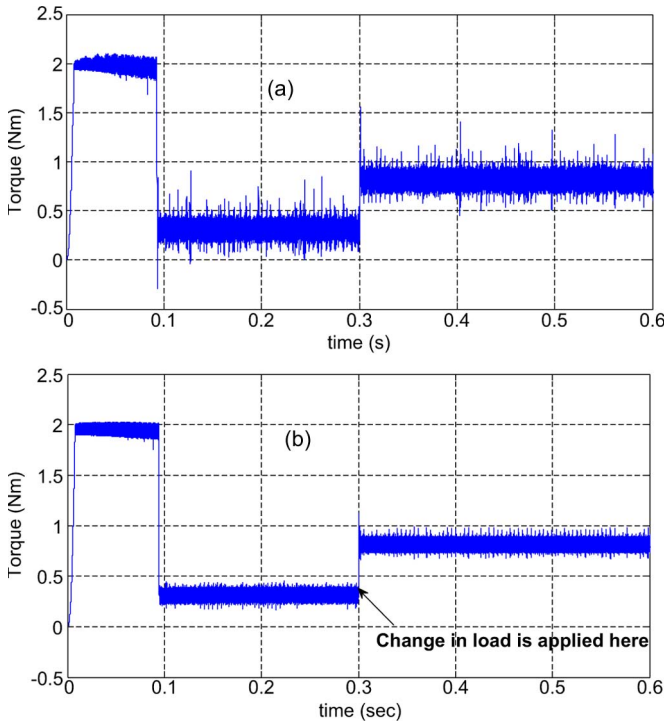
Fig. 9. Developed torque responses of the IM drive for a step change in load from 0.3 to 0.8 N · m at speed of 120 rad/s. (a) Conventional DTC. (b) FLC-based DTC scheme.
