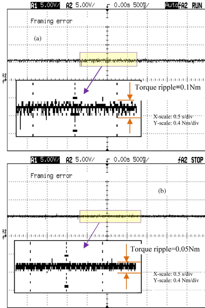
Fig. 16. Steady-state experimental torque responses of the IM drive with zoom-in view of the shaded portion, for command rated speed of 180 rad/s at 0.4 \cdot \text{N} \cdot \text{m} load. (a) Conventional DTC. (b) FLC-based DTC.
