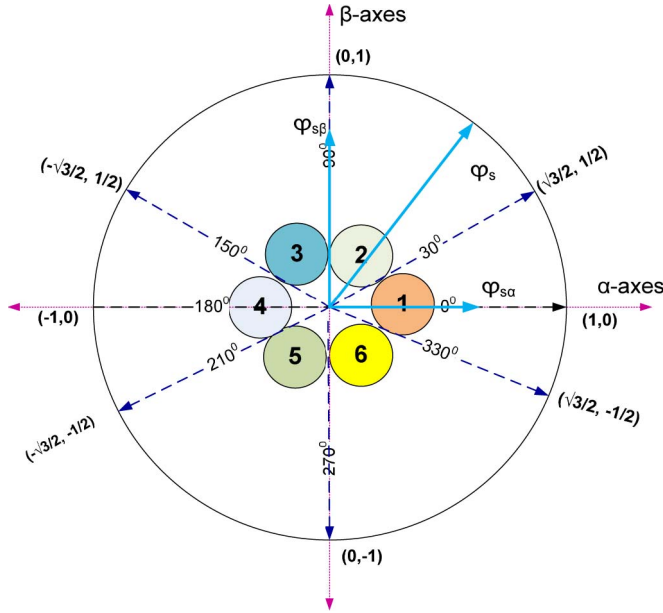
Fig. 3. Stator flux-linkage vector with six sectors. The stator flux-linkage vector with its coordinates is shown at the boundary of each sector.
