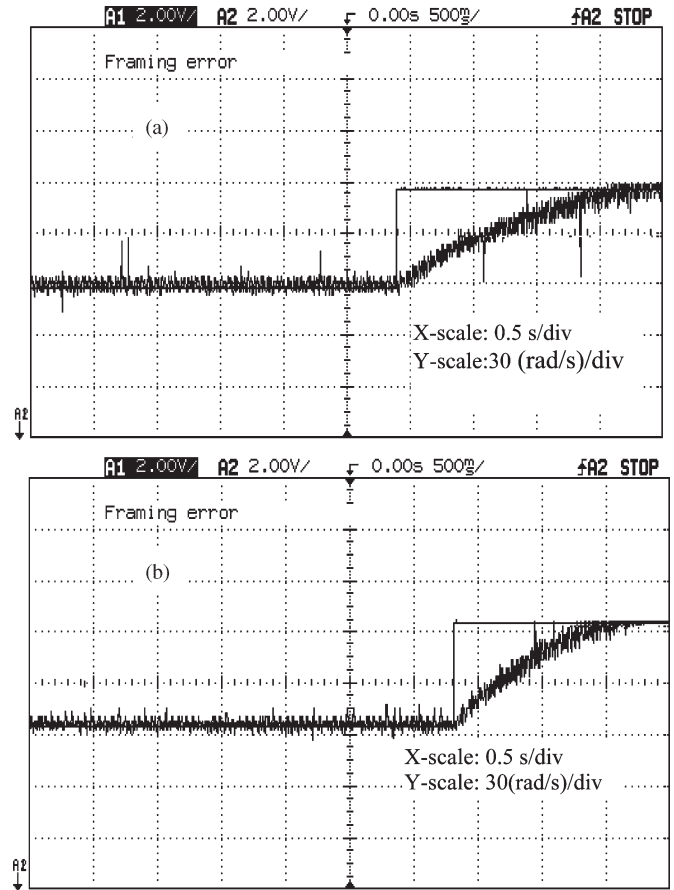
Fig. 17. Speed response for a step change in speed from 120 to 180 rad/s at 0.4 \cdot \text{N} \cdot \text{m} load. (a) Conventional DTC. (b) FLC-based DTC.
