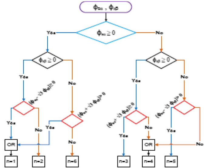
Fig. 4. Flow diagram for flux sector number determination.
