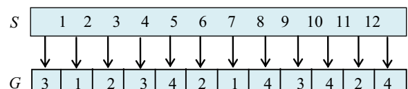
Fig. 4. Generated chromosome from Table 1.
