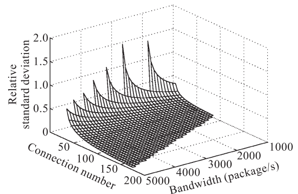
Fig. 3 Variation of the queue length relative standard deviation for various n and C
