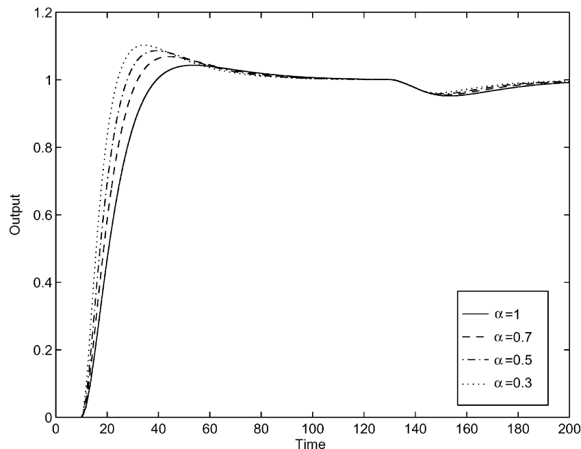
Fig. 5. Responses for Example 1.
