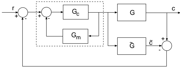
Fig. 3. IMC representation of a Smith predictor.
